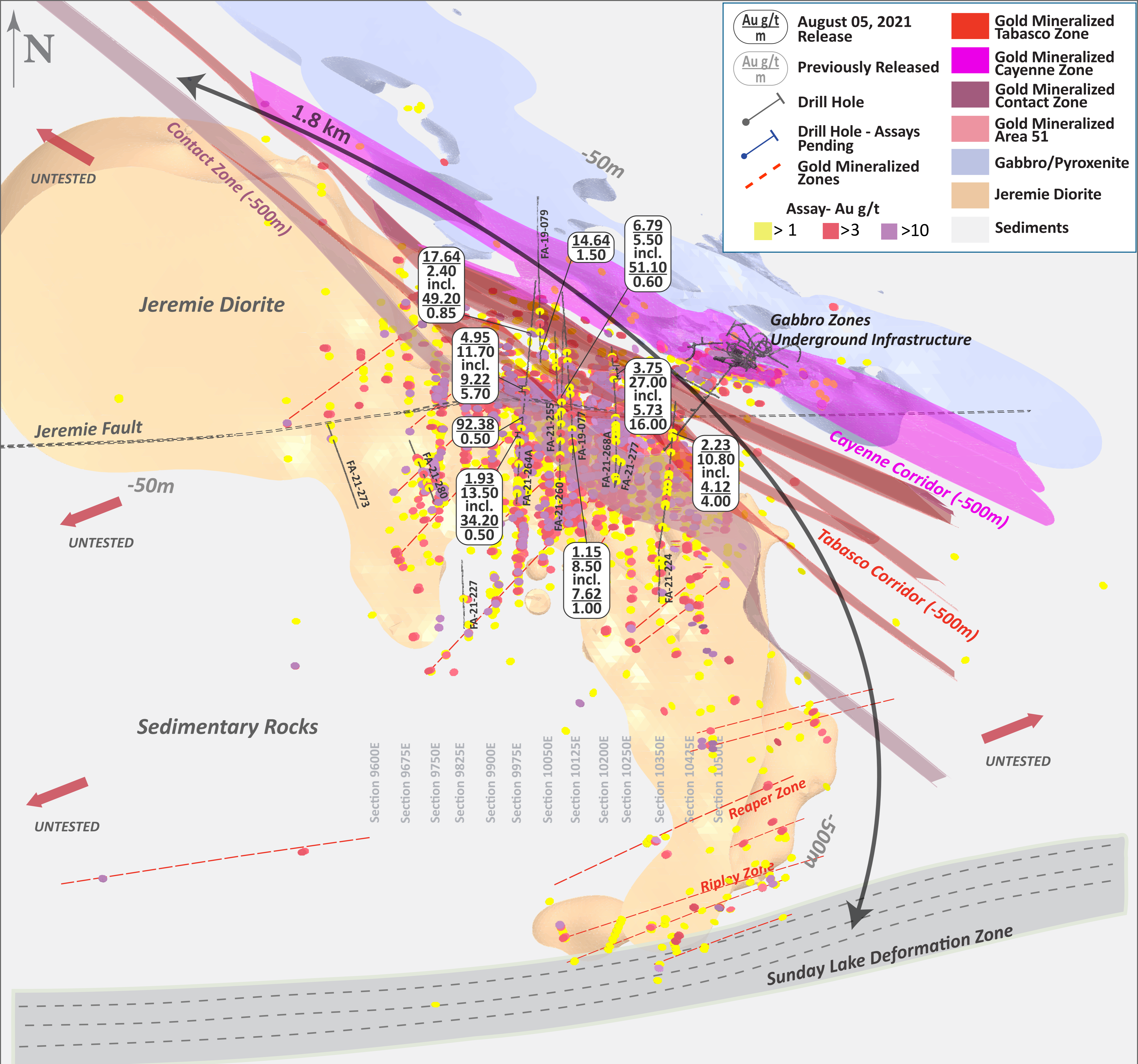
Fenelon Gold System Plan View August 05, 2021
