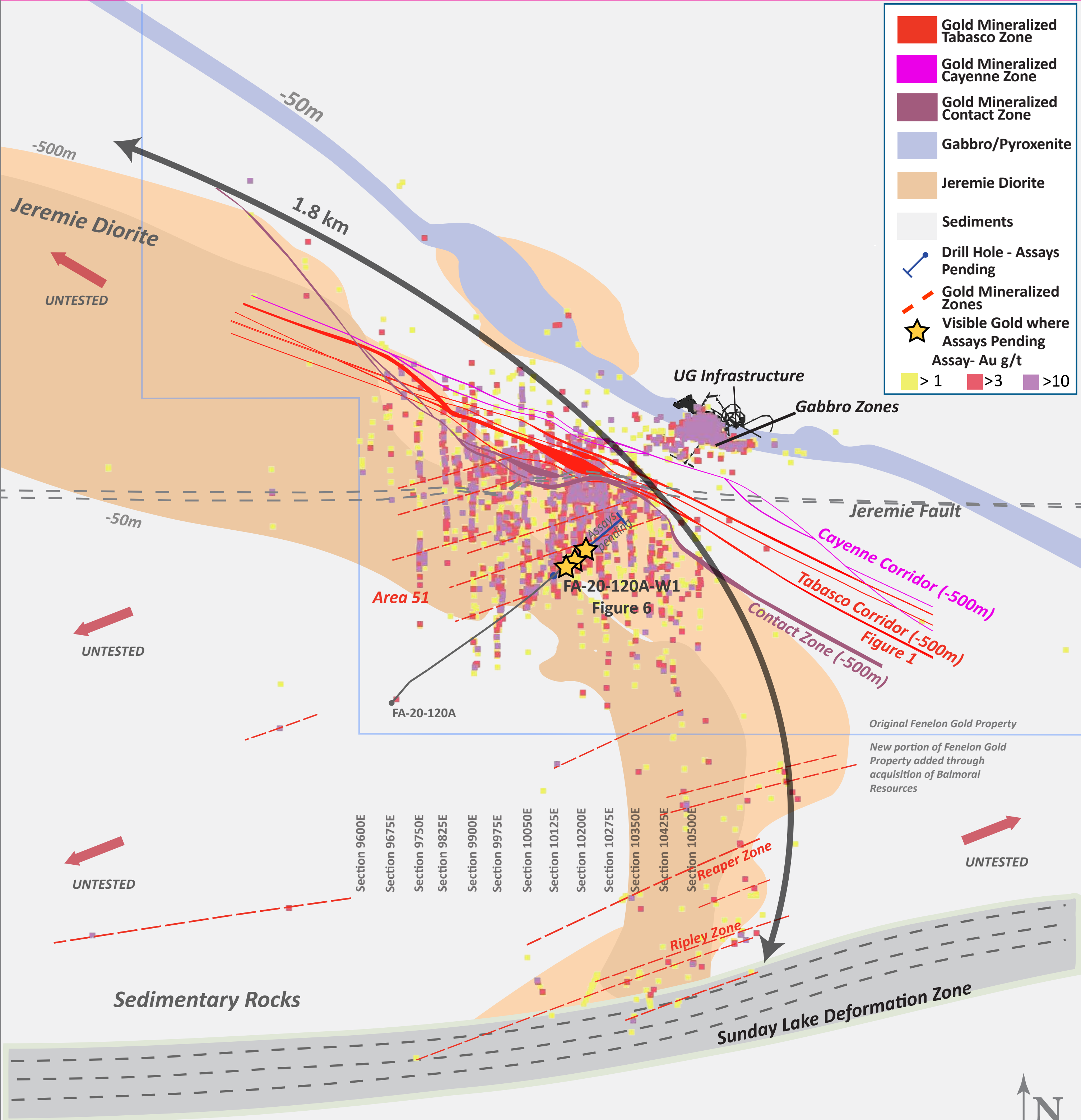
Fenelon Gold System Plan View February 17, 2021
